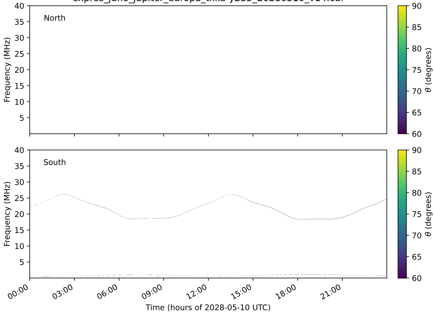
expres_juno_jupiter_europa_txka-y235_20280510_v14.cdf
