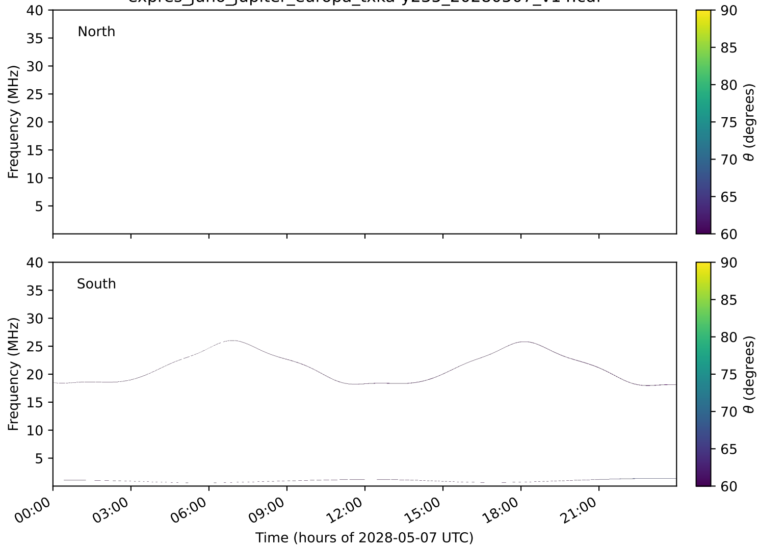
expres_juno_jupiter_europa_txka-y235_20280507_v14.cdf
