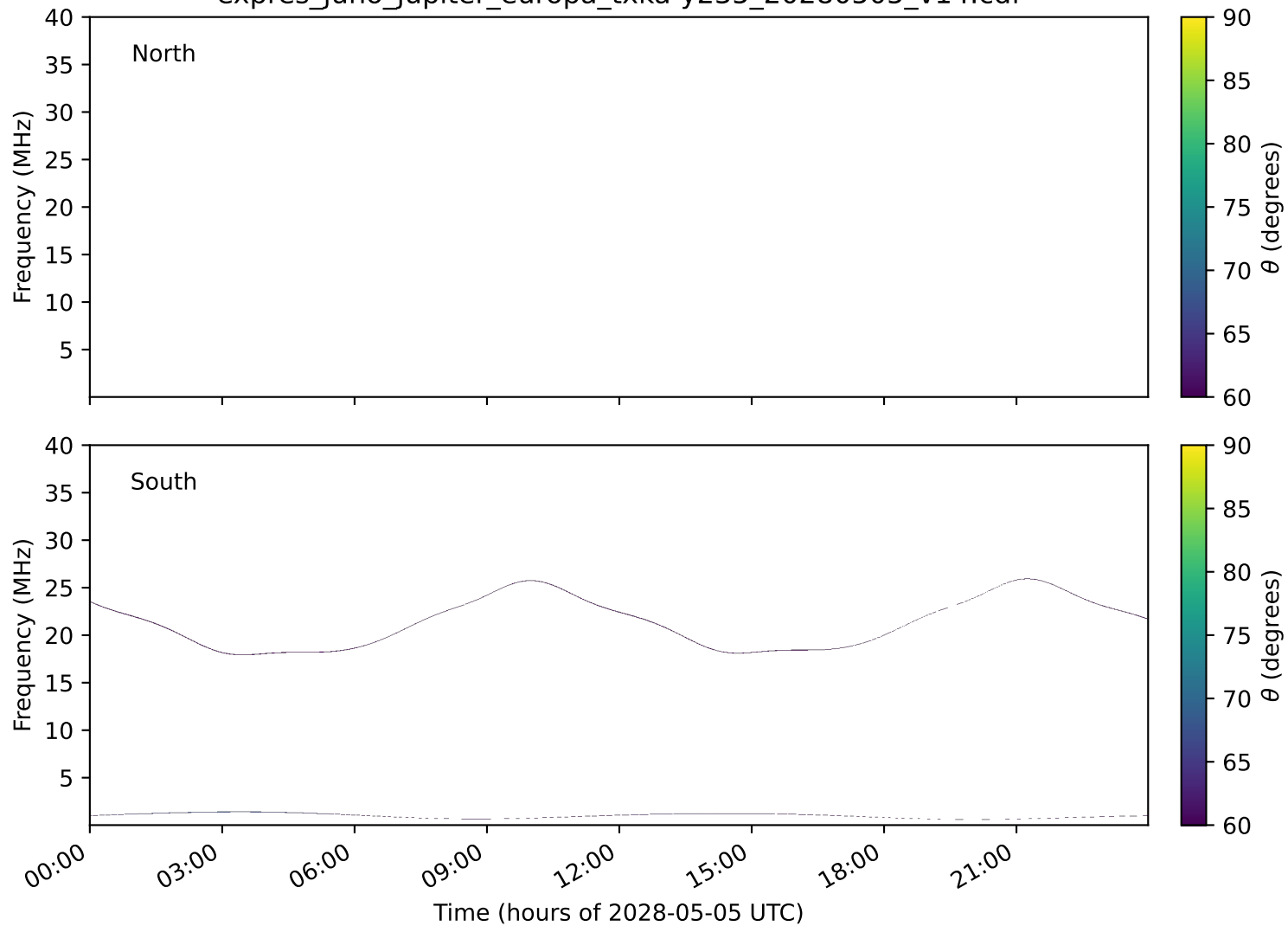
expres_juno_jupiter_europa_txka-y235_20280505_v14.cdf
