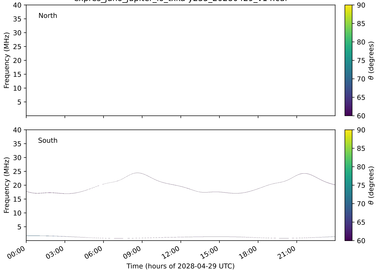
expres_juno_jupiter_io_txka-y235_20280429_v14.cdf
