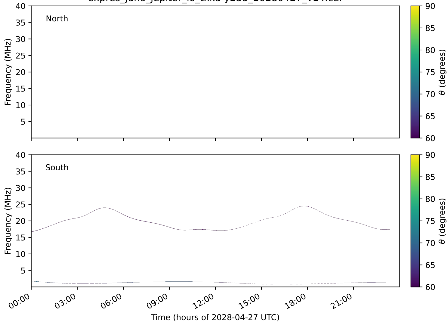
expres_juno_jupiter_io_txka-y235_20280427_v14.cdf
