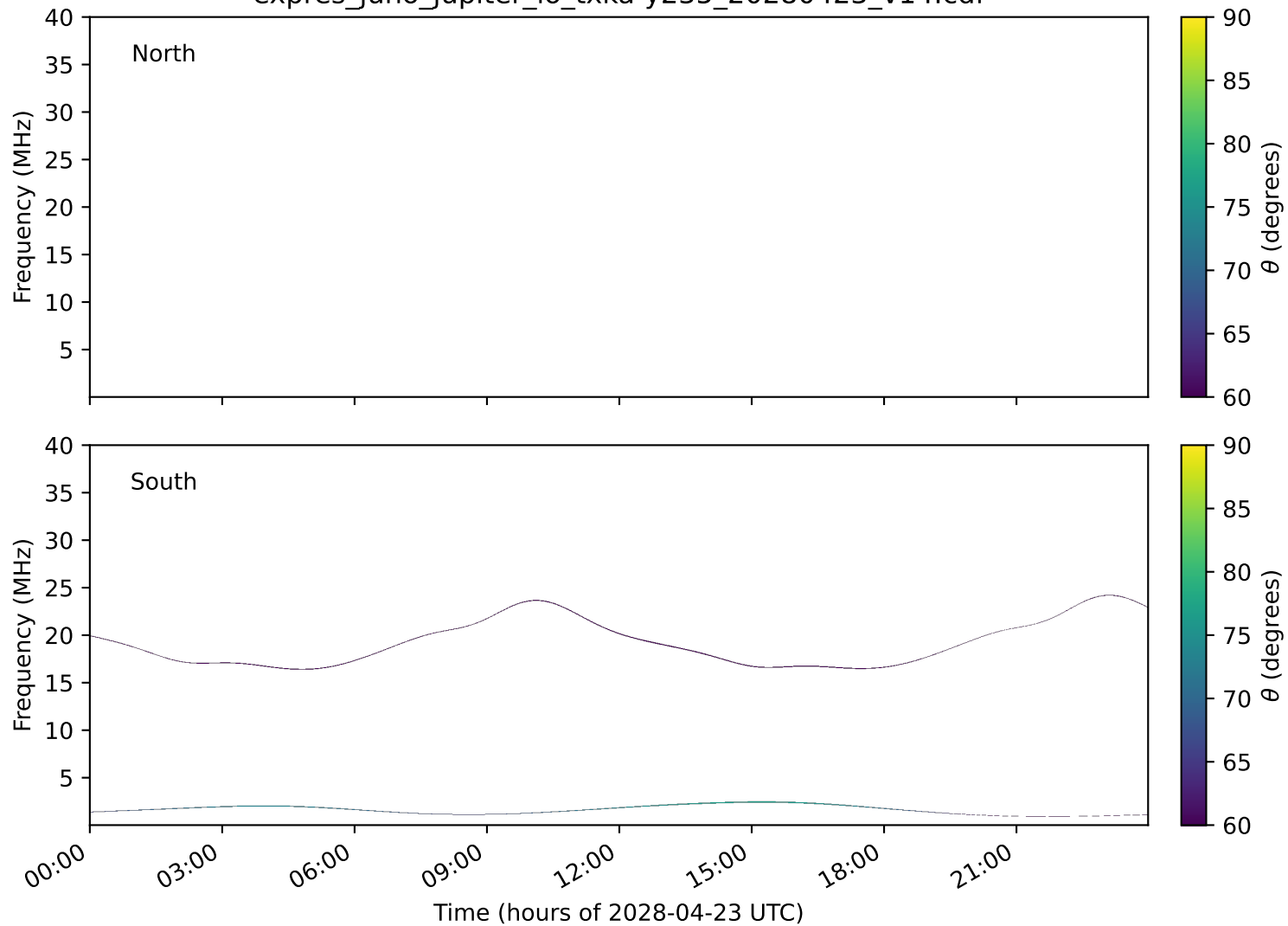
expres_juno_jupiter_io_txka-y235_20280423_v14.cdf
