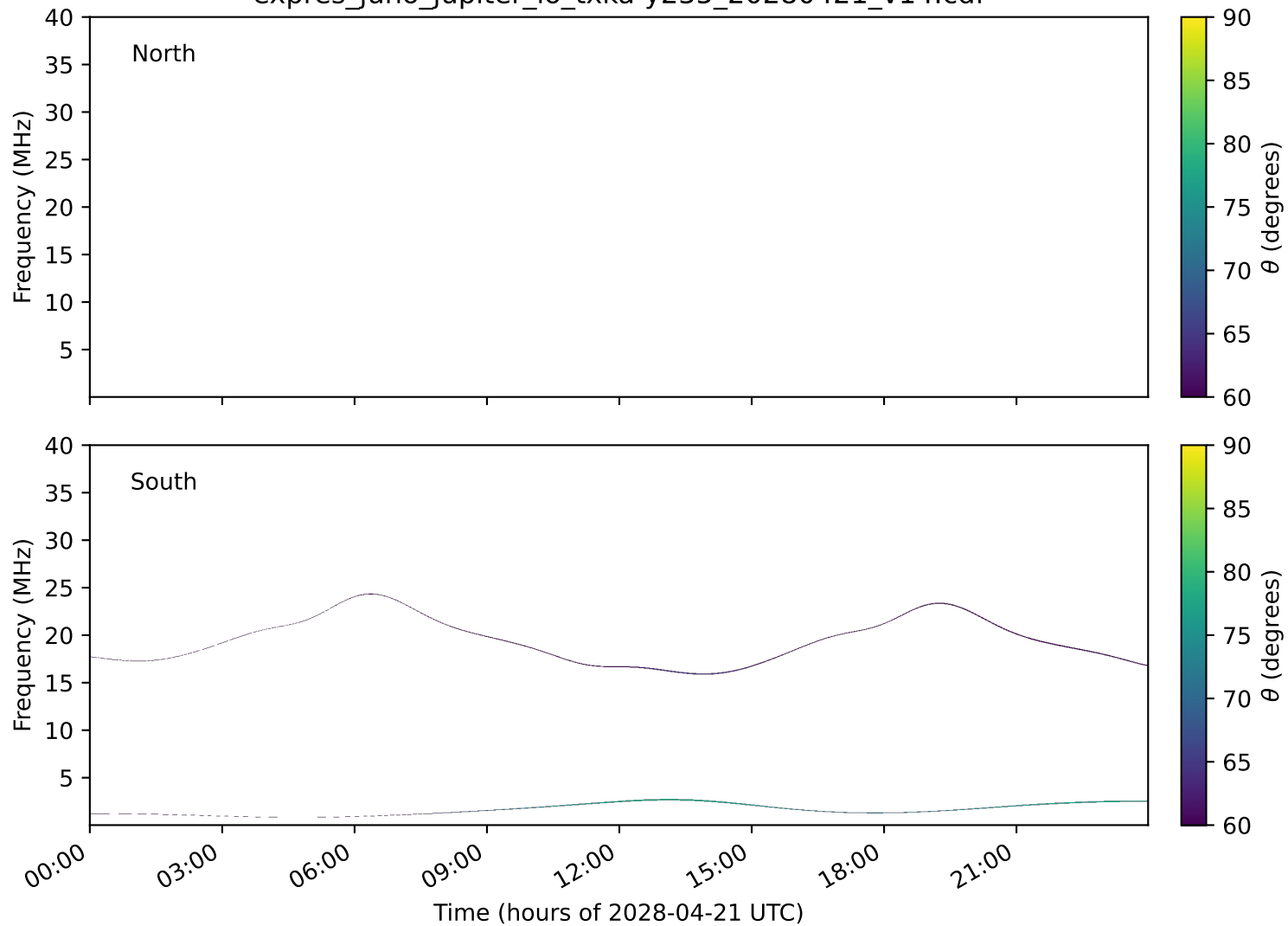
expres_juno_jupiter_io_txka-y235_20280421_v14.cdf
