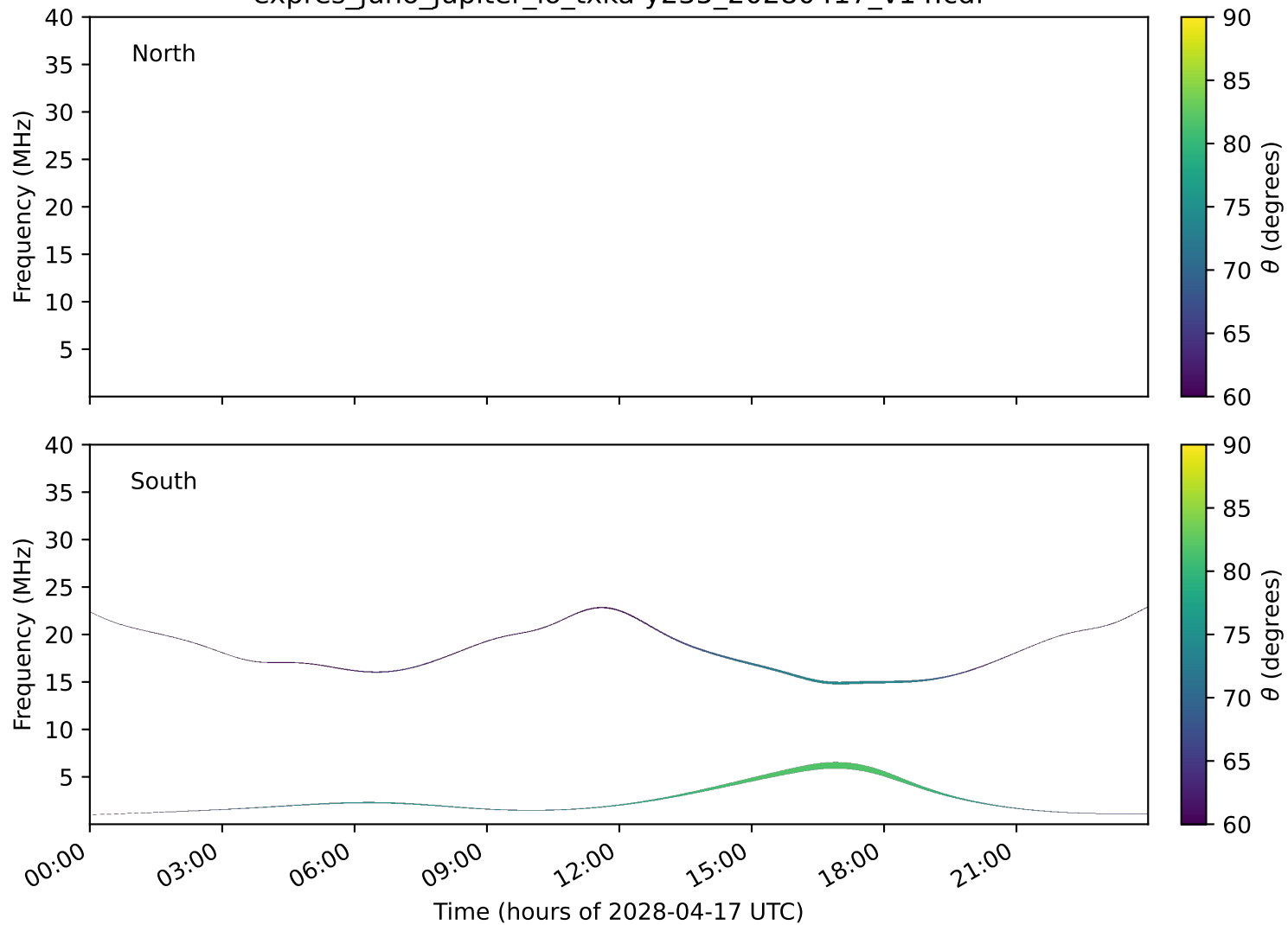
expres_juno_jupiter_io_txka-y235_20280417_v14.cdf
