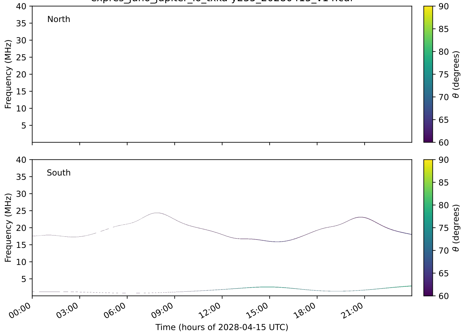
expres_juno_jupiter_io_txka-y235_20280415_v14.cdf
