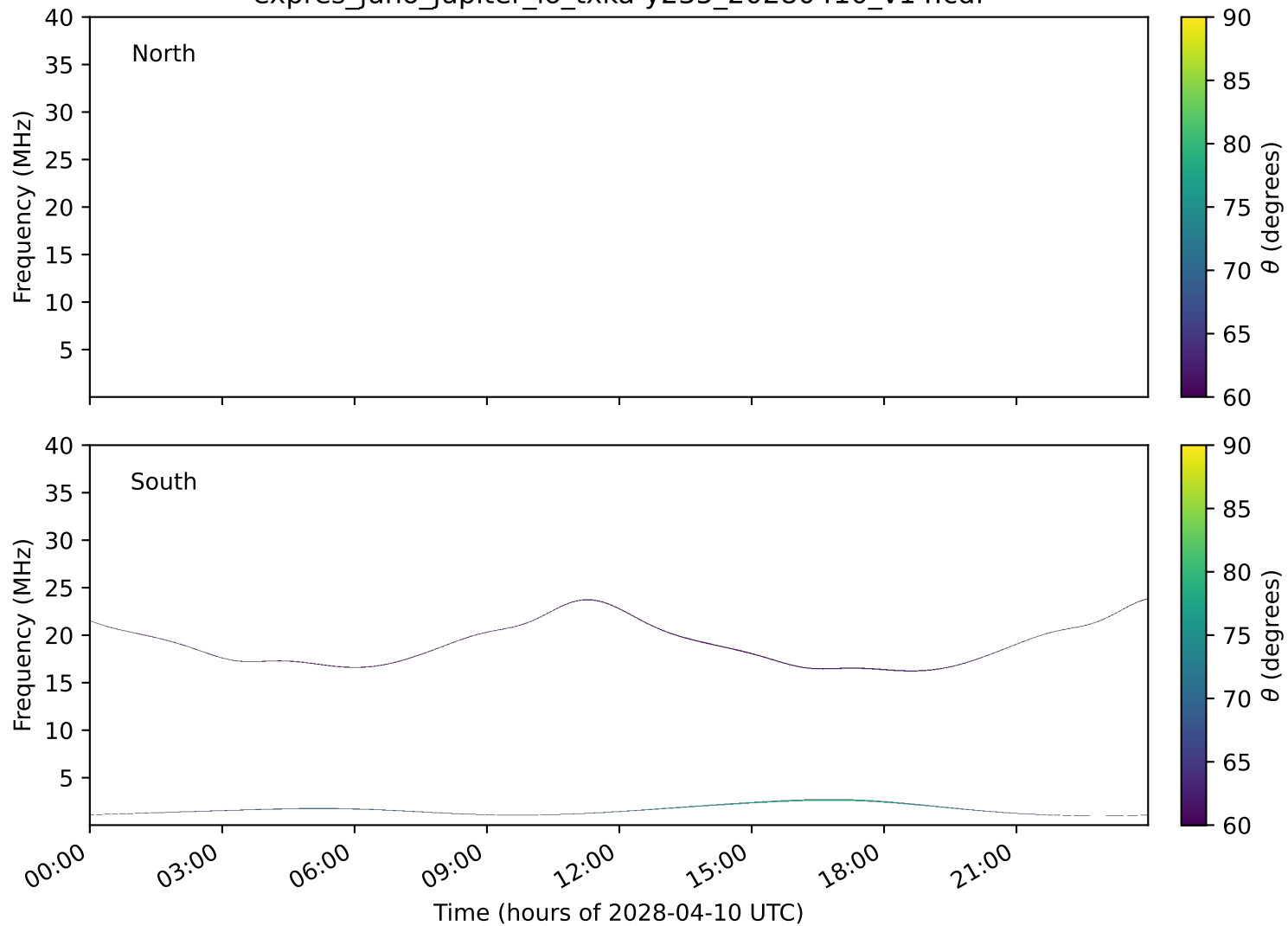
expres_juno_jupiter_io_txka-y235_20280410_v14.cdf
