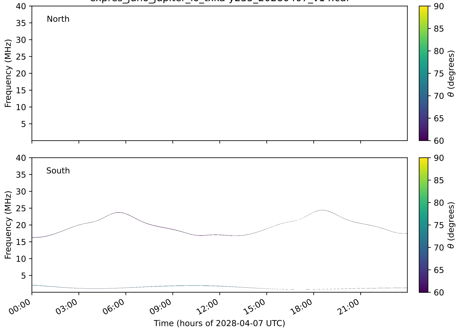
expres_juno_jupiter_io_txka-y235_20280407_v14.cdf
