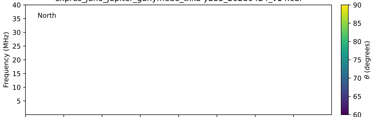
expres_juno_jupiter_ganymede_txka-y235_20280424_v14.cdf
