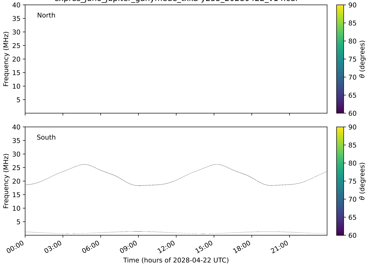
expres_juno_jupiter_ganymede_txka-y235_20280422_v14.cdf
