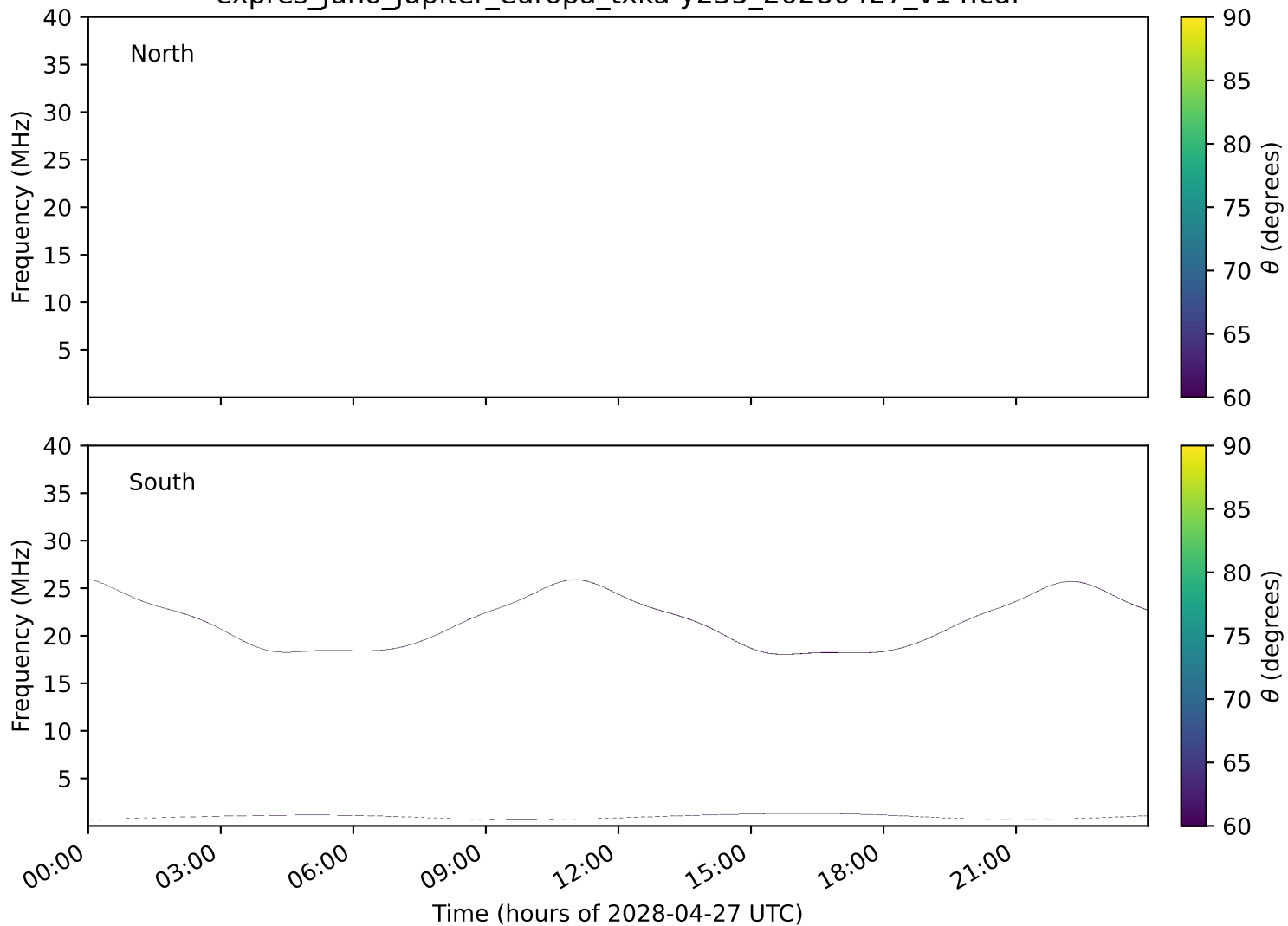
expres_juno_jupiter_europa_txka-y235_20280427_v14.cdf
