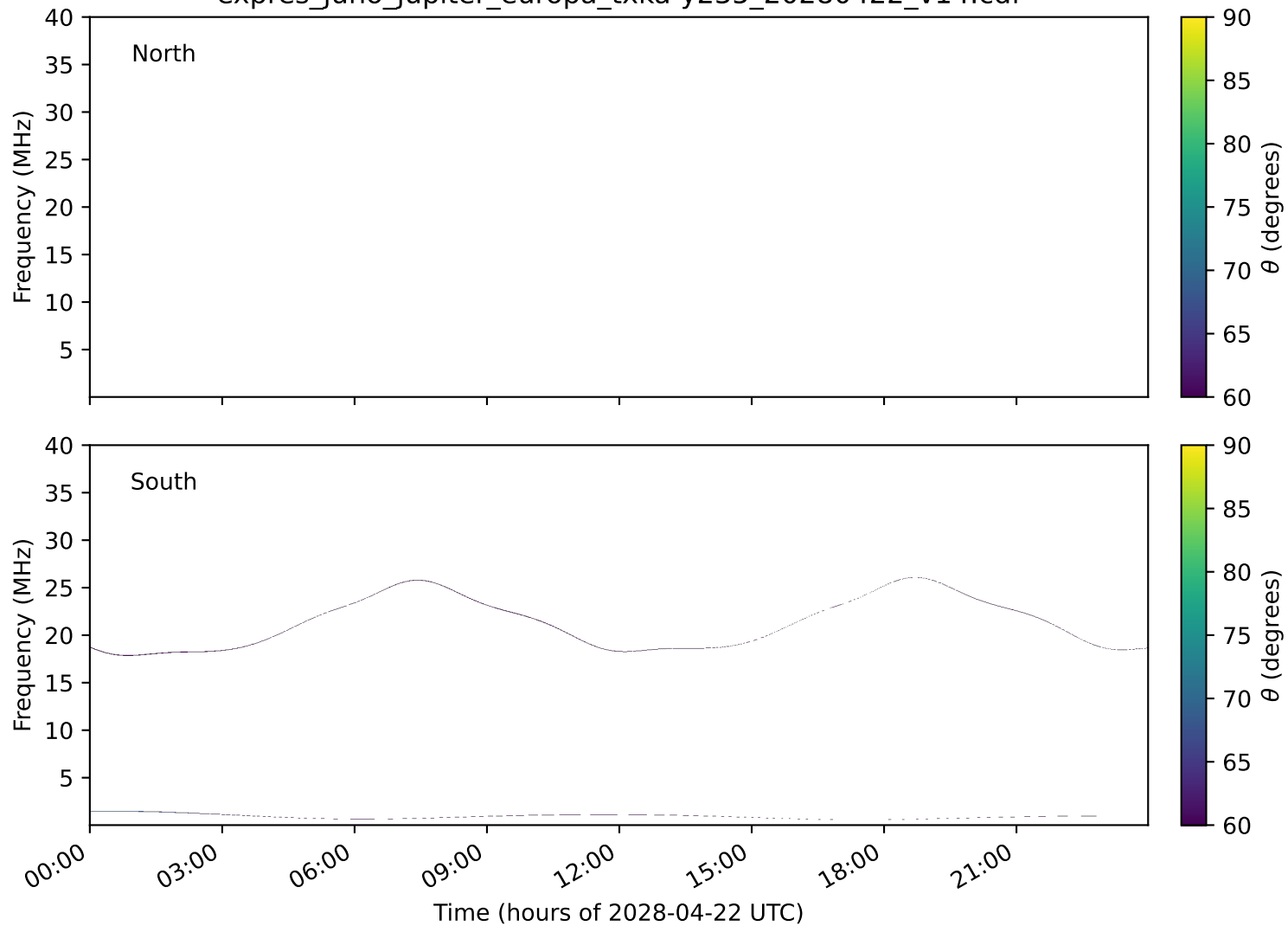
expres_juno_jupiter_europa_txka-y235_20280422_v14.cdf
