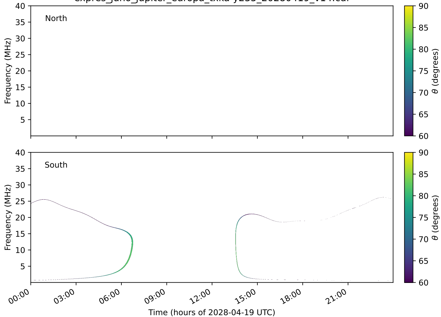
expres_juno_jupiter_europa_txka-y235_20280419_v14.cdf
