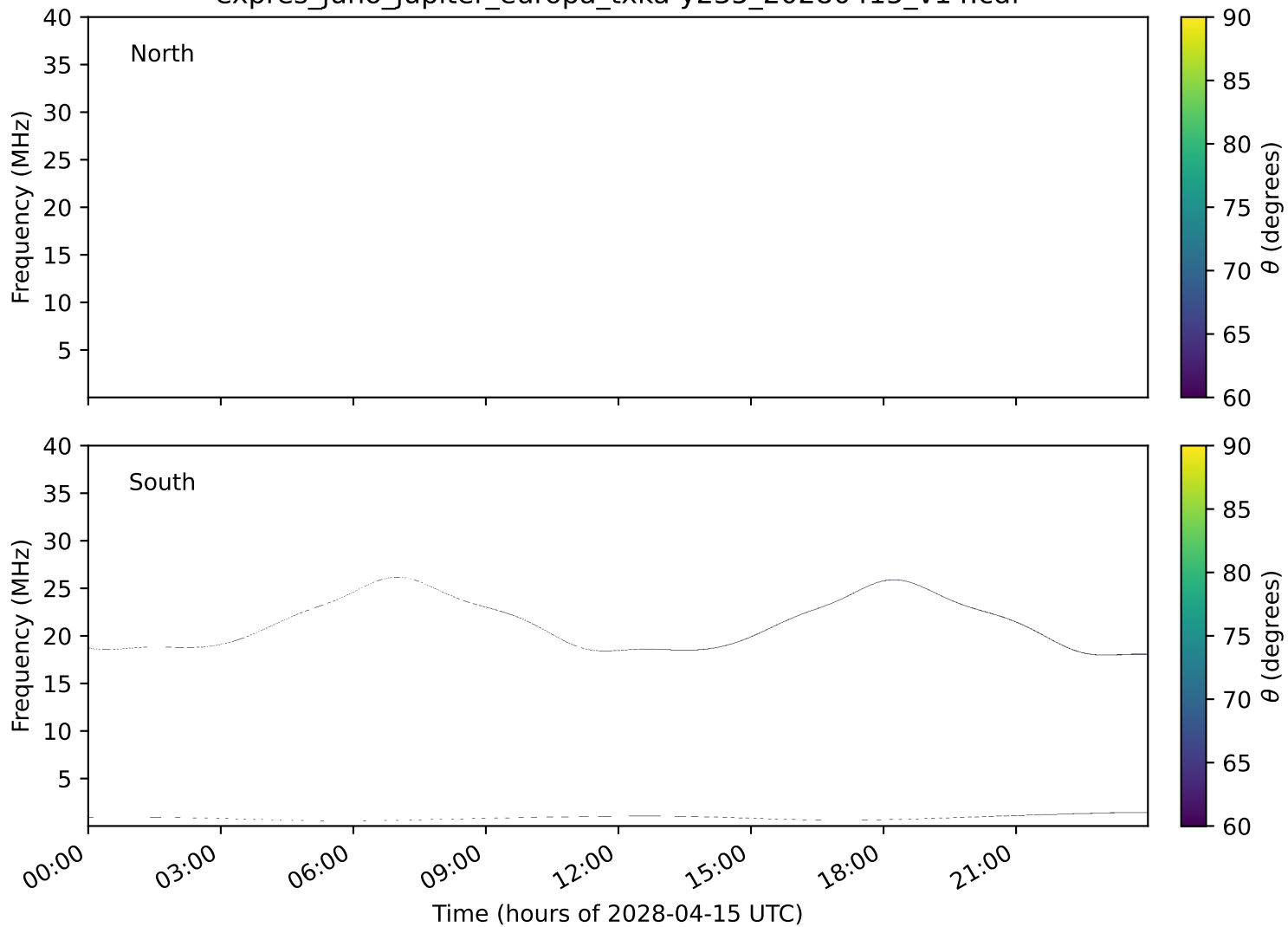
expres_juno_jupiter_europa_txka-y235_20280415_v14.cdf
