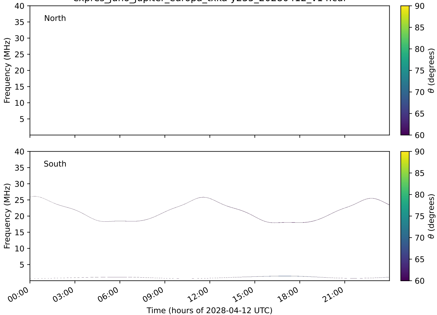
expres_juno_jupiter_europa_txka-y235_20280412_v14.cdf
