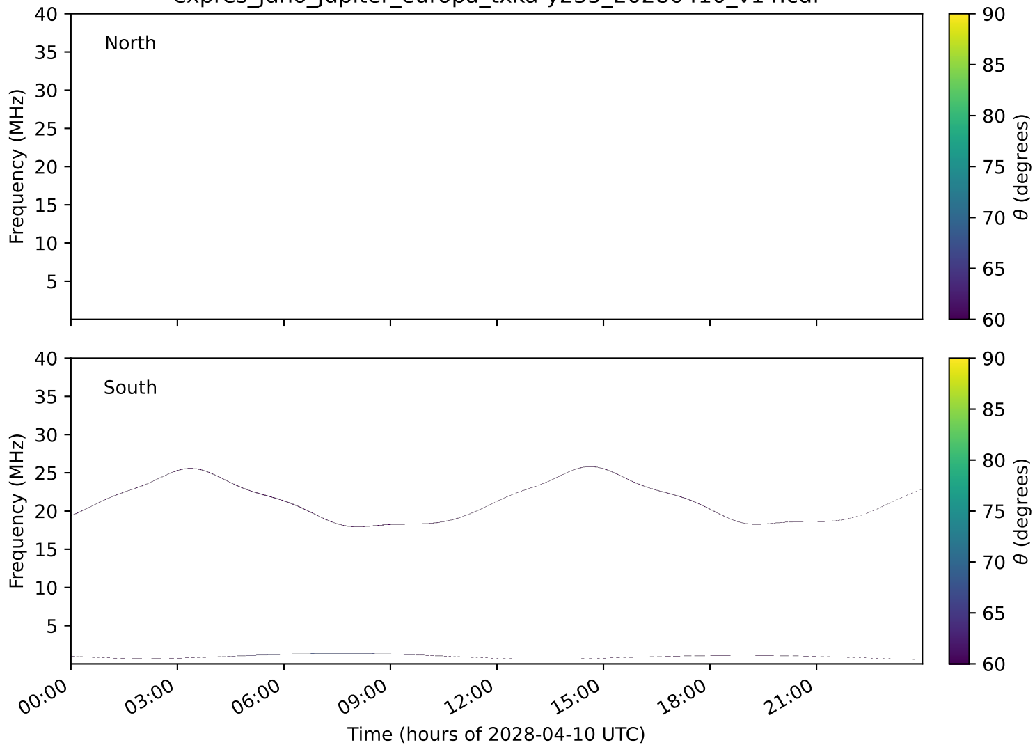
expres_juno_jupiter_europa_txka-y235_20280410_v14.cdf
