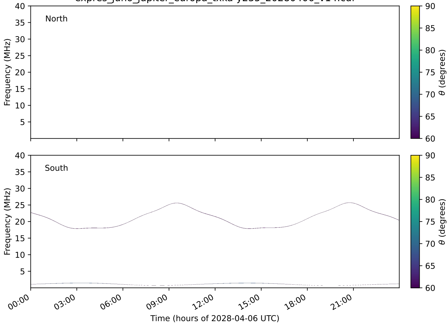
expres_juno_jupiter_europa_txka-y235_20280406_v14.cdf
