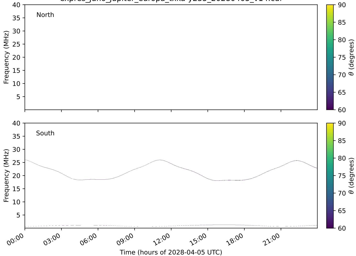
expres_juno_jupiter_europa_txka-y235_20280405_v14.cdf
