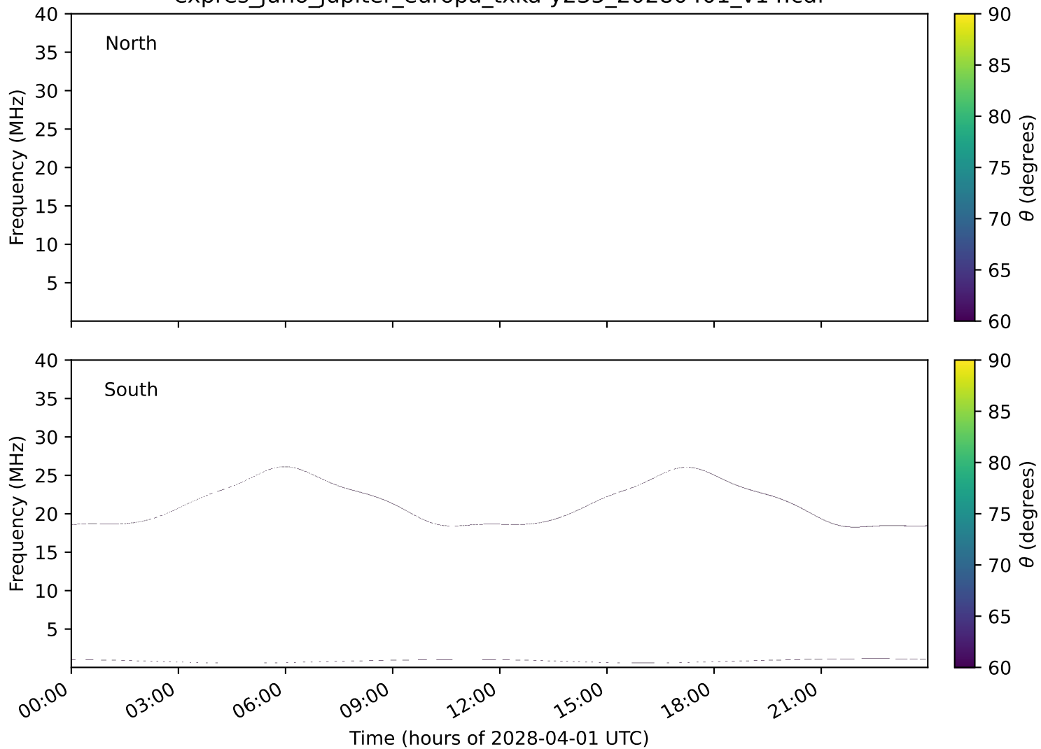
expres_juno_jupiter_europa_txka-y235_20280401_v14.cdf
