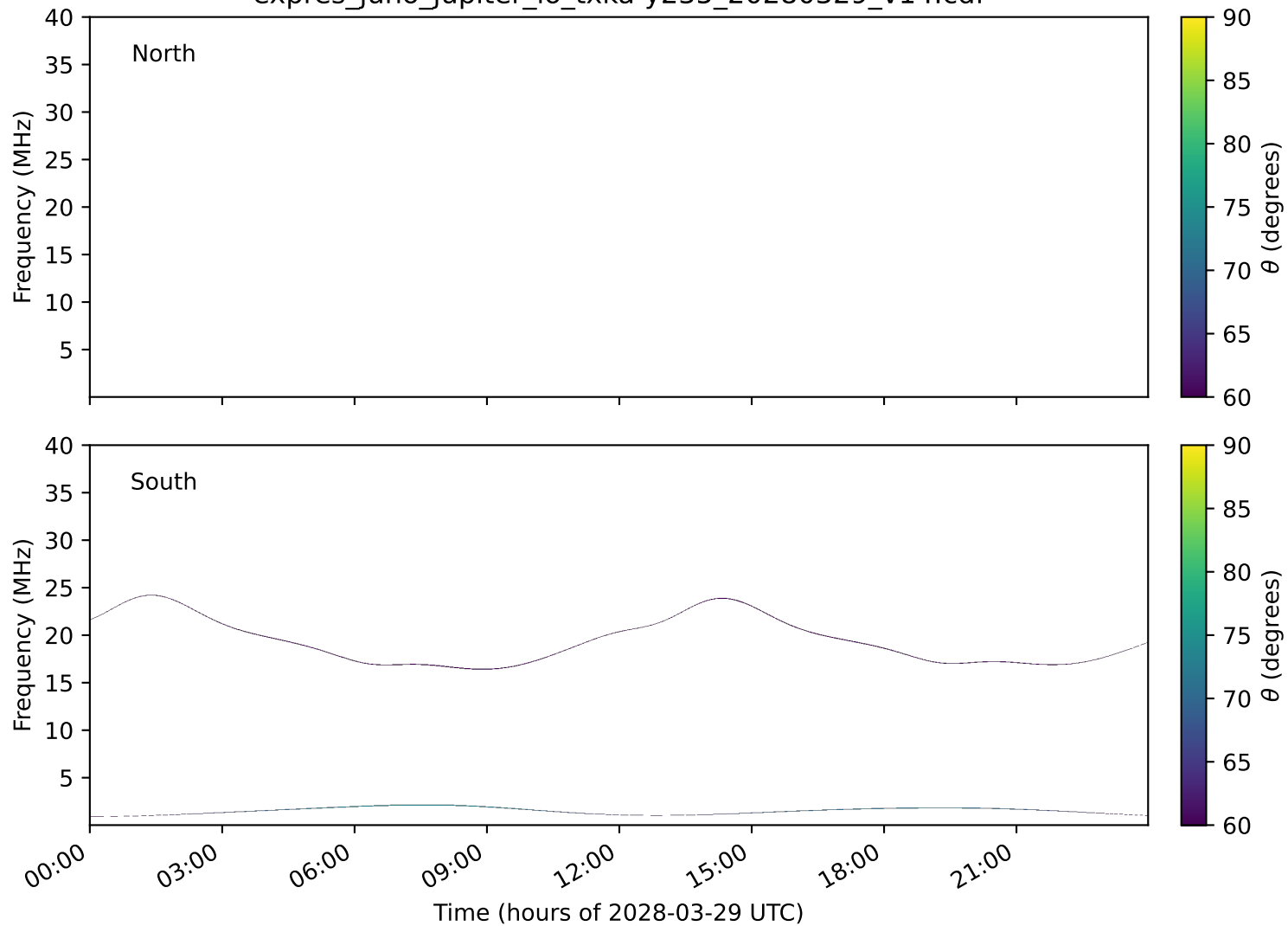
expres_juno_jupiter_io_txka-y235_20280329_v14.cdf
