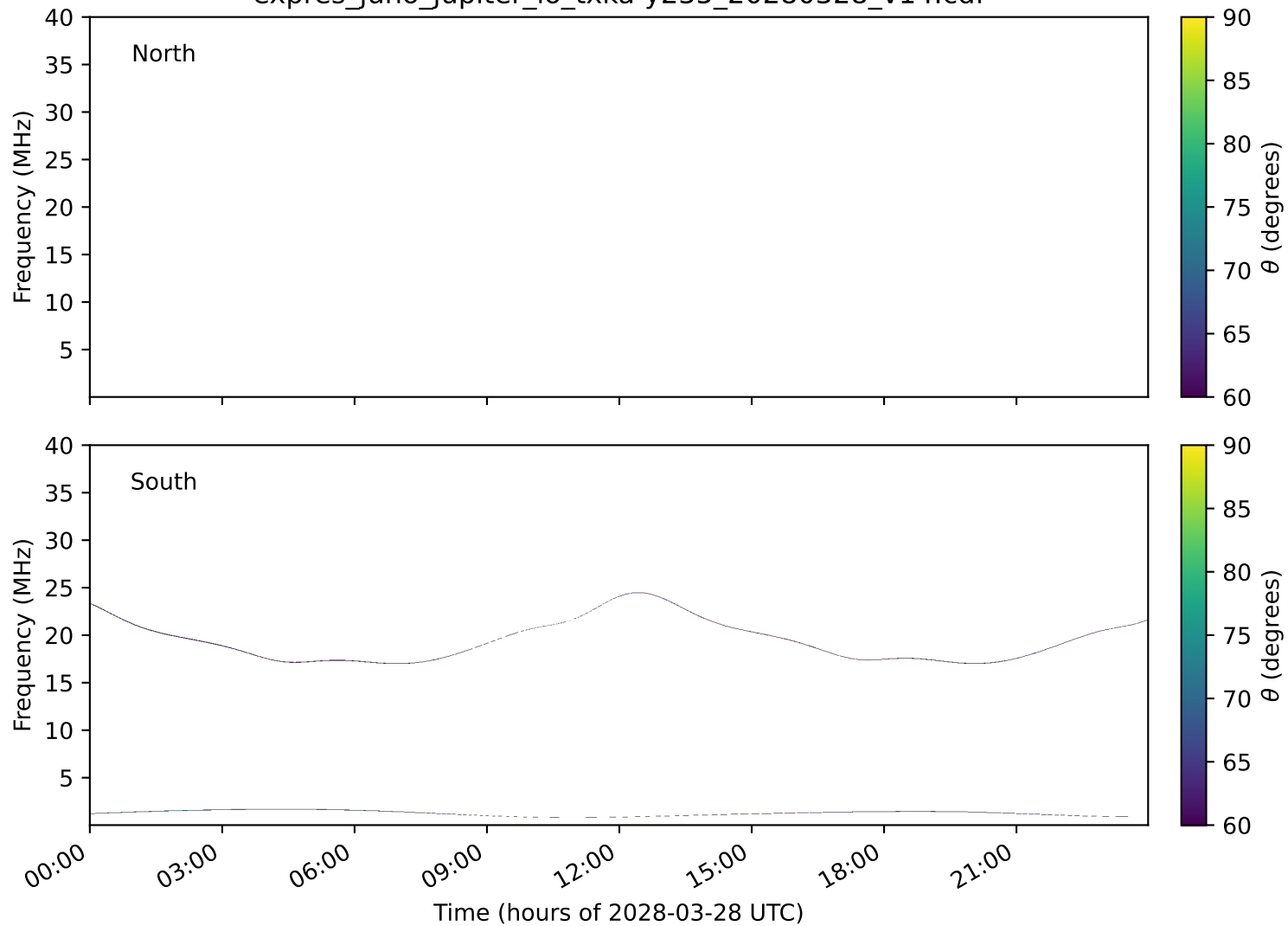
expres_juno_jupiter_io_txka-y235_20280328_v14.cdf
