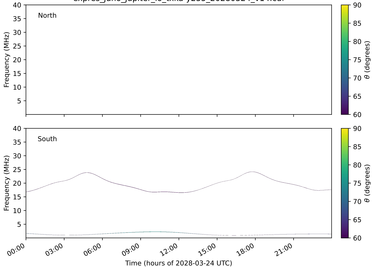
expres_juno_jupiter_io_txka-y235_20280324_v14.cdf
