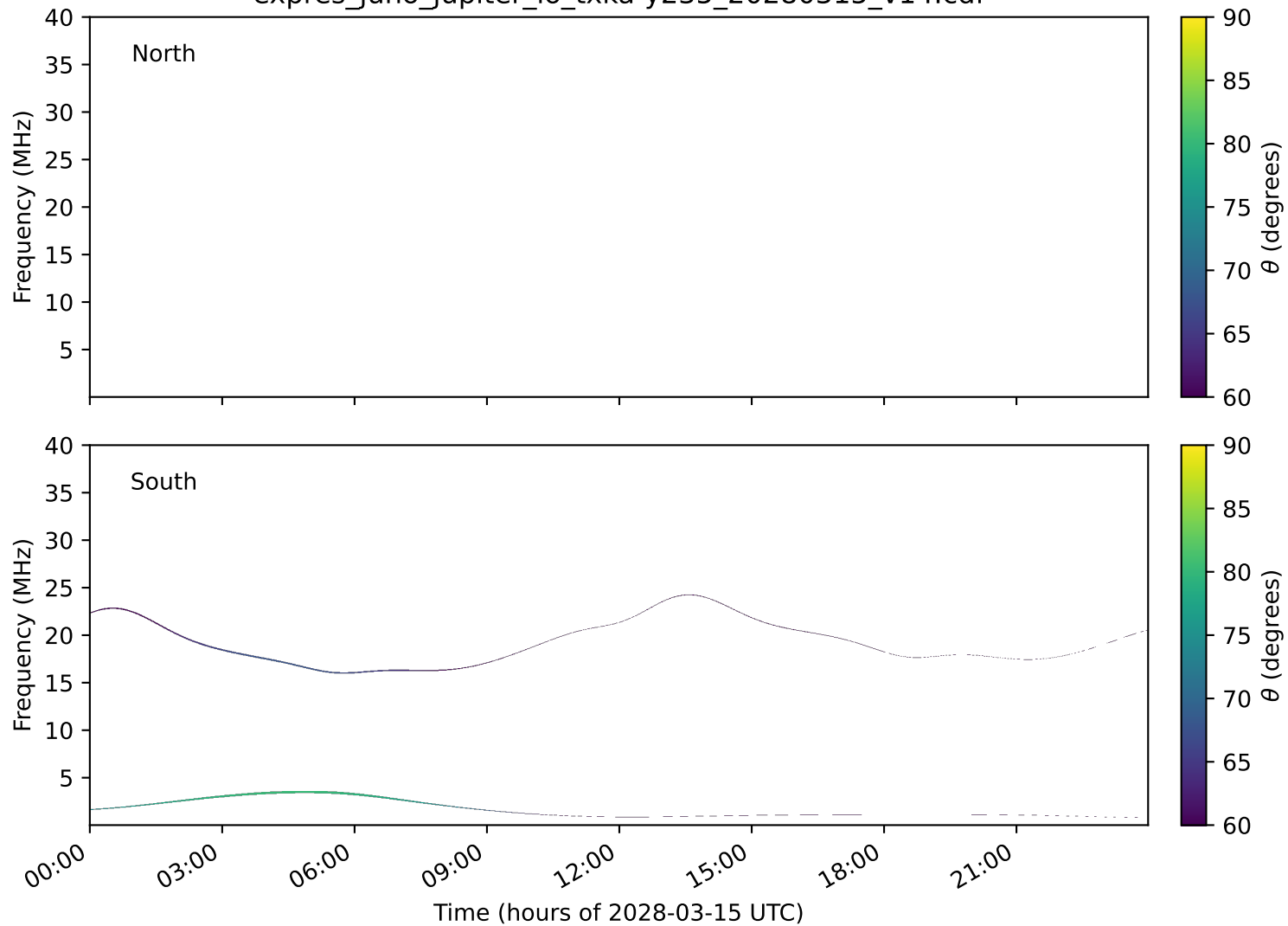
expres_juno_jupiter_io_txka-y235_20280315_v14.cdf
