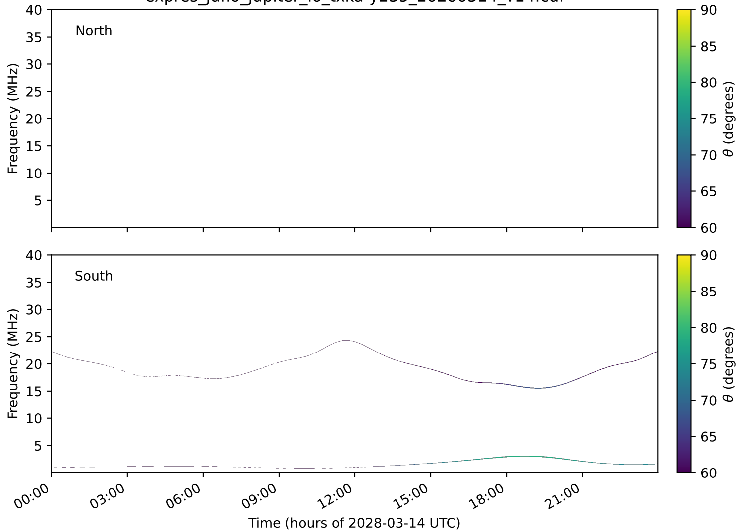
expres_juno_jupiter_io_txka-y235_20280314_v14.cdf
