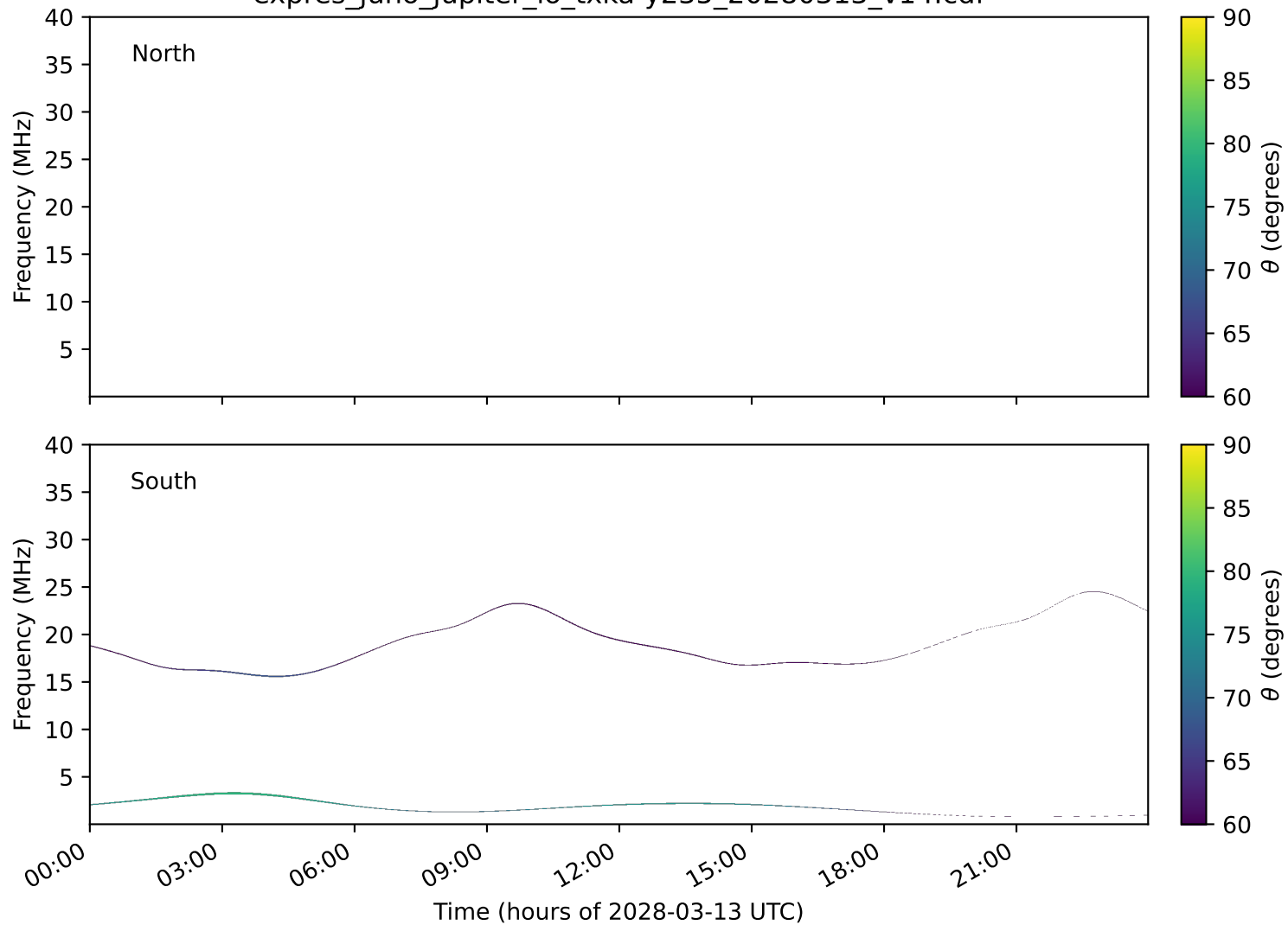
expres_juno_jupiter_io_txka-y235_20280313_v14.cdf
