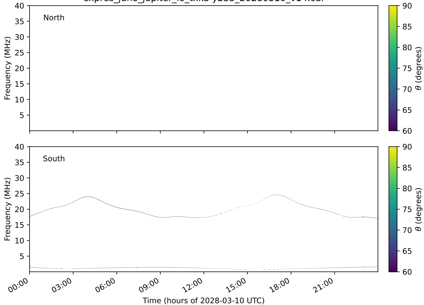
expres_juno_jupiter_io_txka-y235_20280310_v14.cdf
