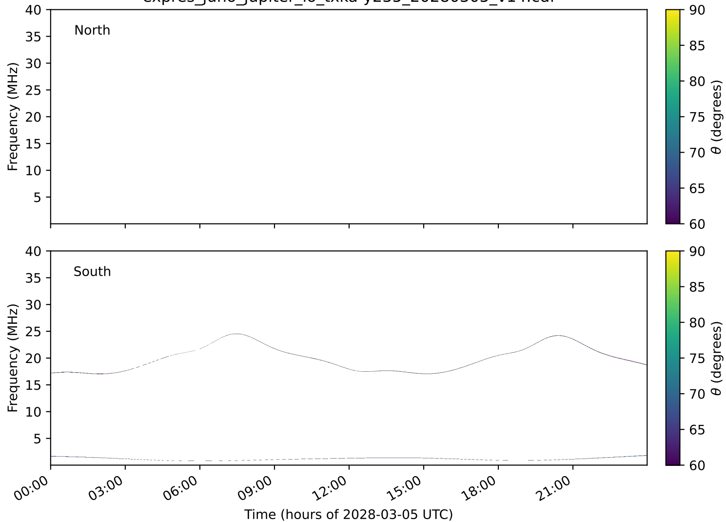
expres_juno_jupiter_io_txka-y235_20280305_v14.cdf
