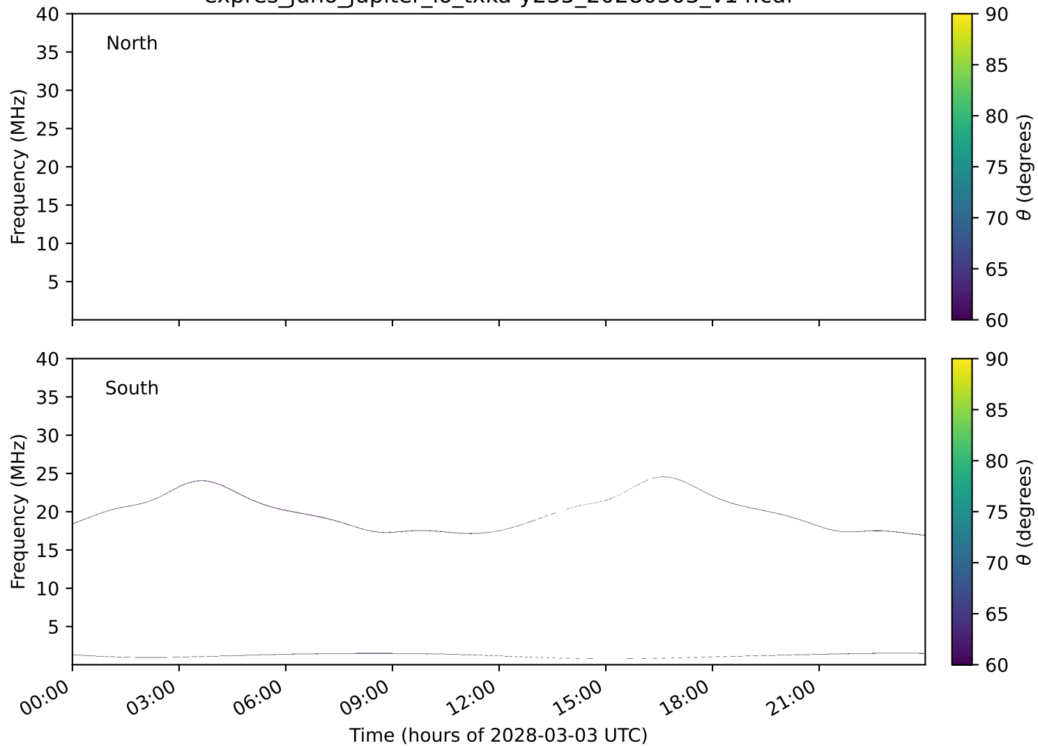
expres_juno_jupiter_io_txka-y235_20280303_v14.cdf
