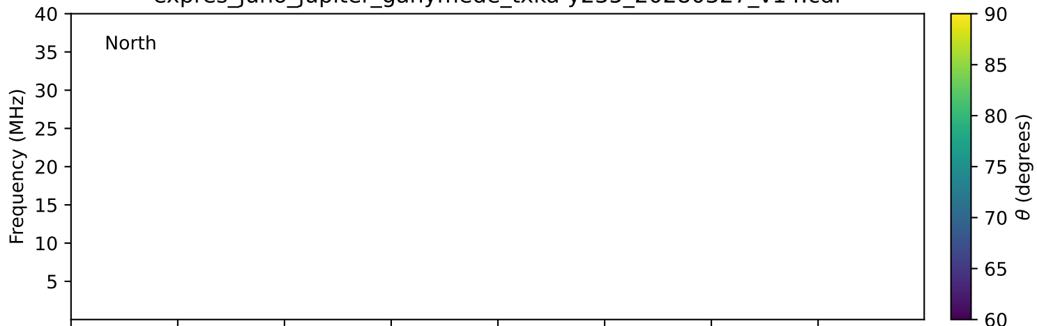
expres_juno_jupiter_ganymede_txka-y235_20280327_v14.cdf
