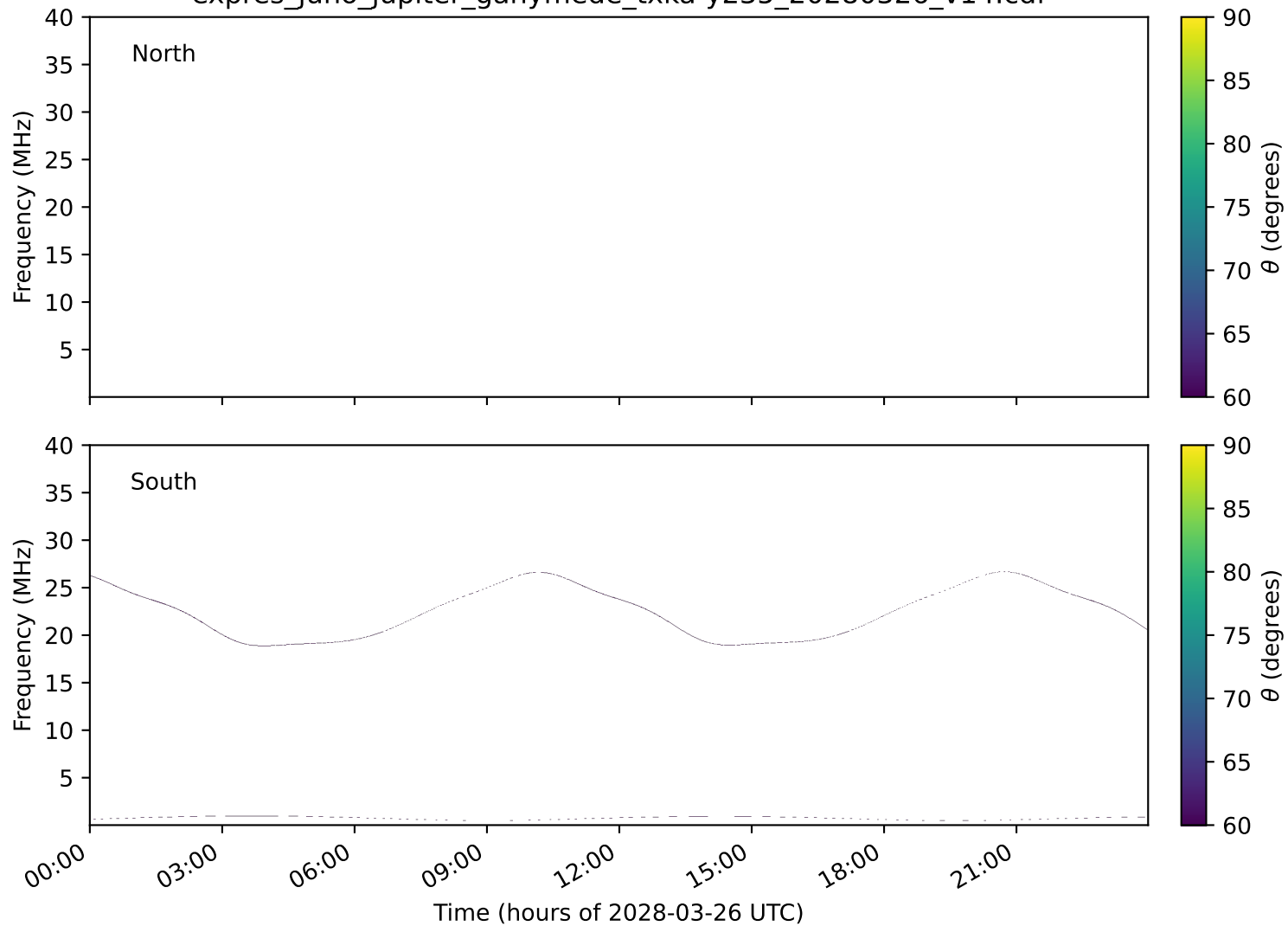
expres_juno_jupiter_ganymede_txka-y235_20280326_v14.cdf
