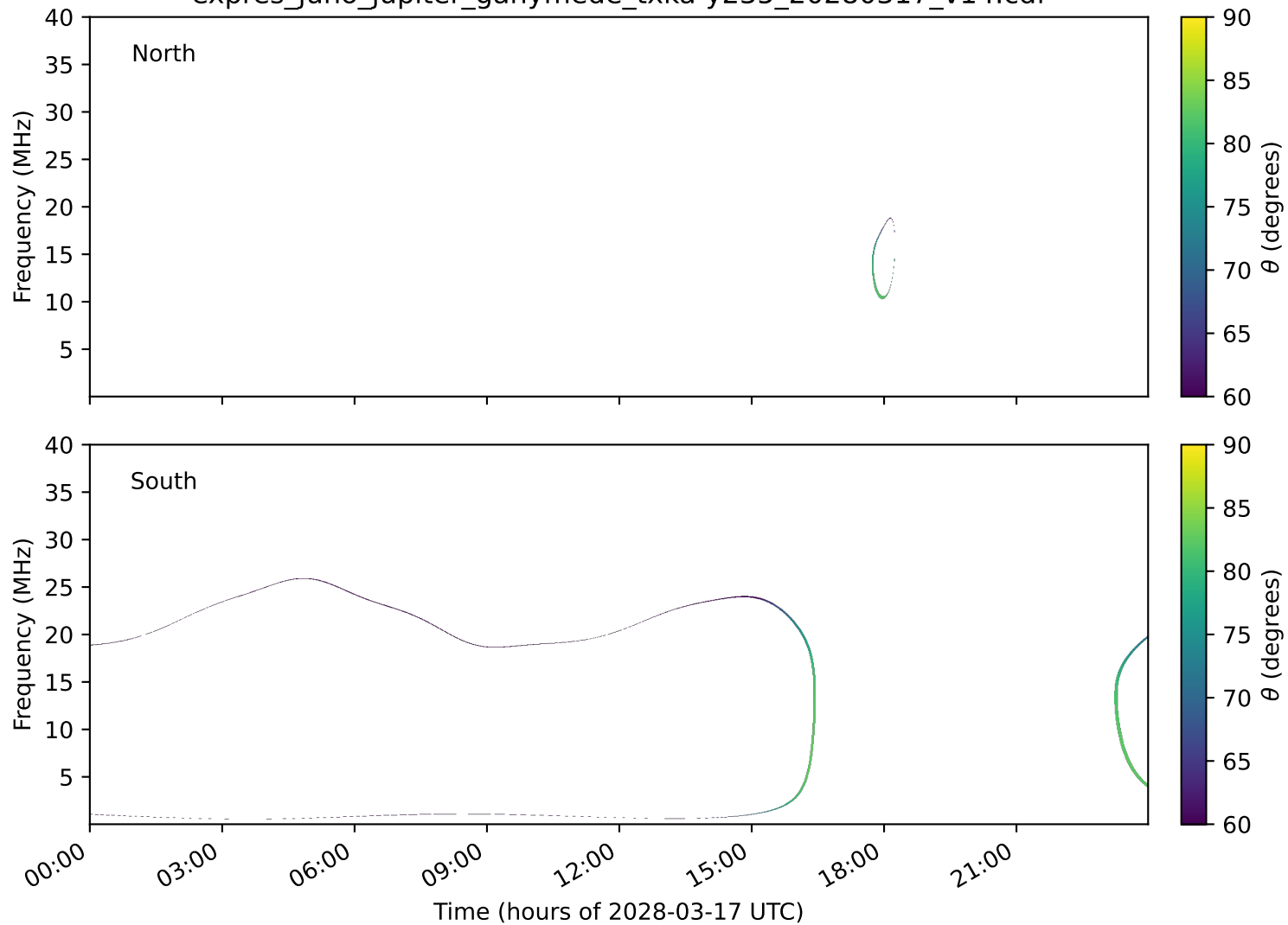
expres_juno_jupiter_ganymede_txka-y235_20280317_v14.cdf
