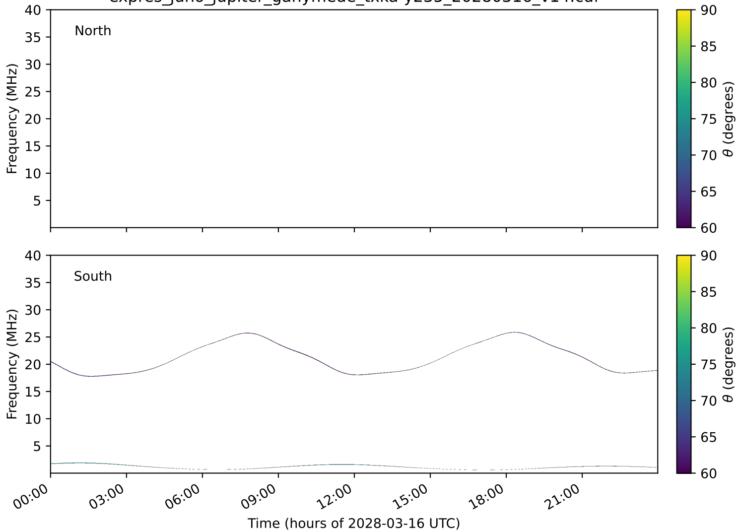
expres_juno_jupiter_ganymede_txka-y235_20280316_v14.cdf
