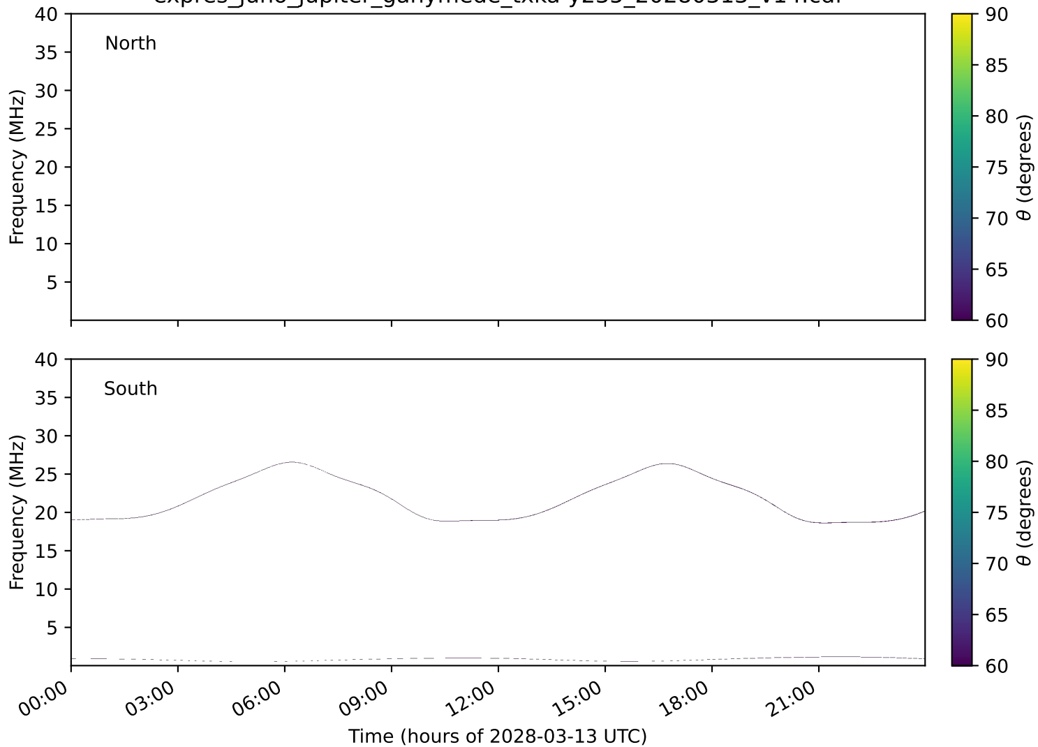
expres_juno_jupiter_ganymede_txka-y235_20280313_v14.cdf
