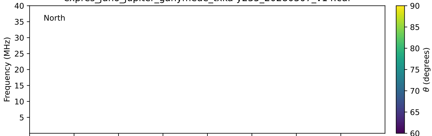
expres_juno_jupiter_ganymede_txka-y235_20280307_v14.cdf
