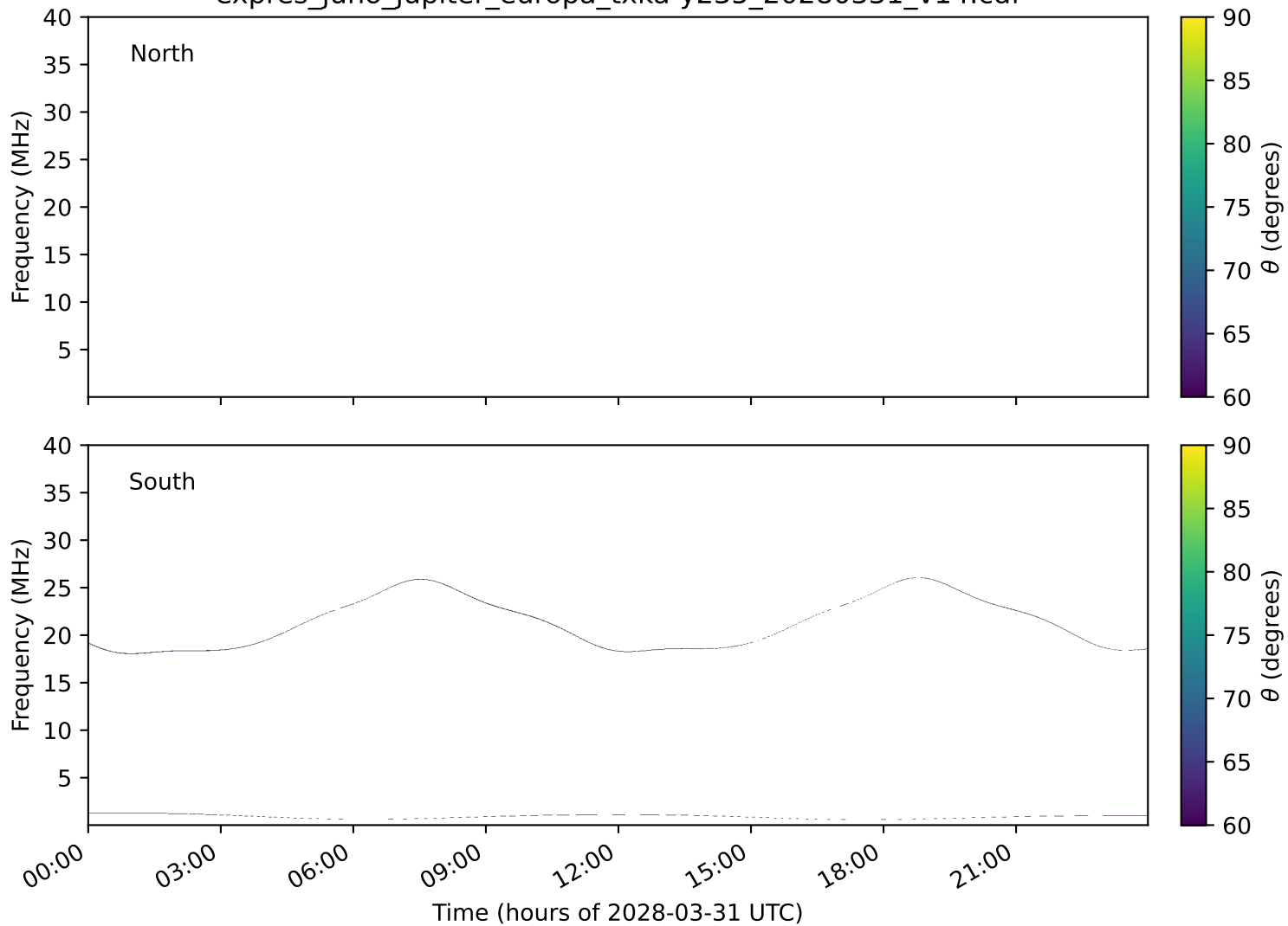
expres_juno_jupiter_europa_txka-y235_20280331_v14.cdf
