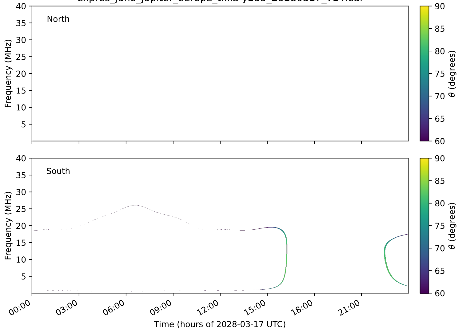
expres_juno_jupiter_europa_txka-y235_20280317_v14.cdf
