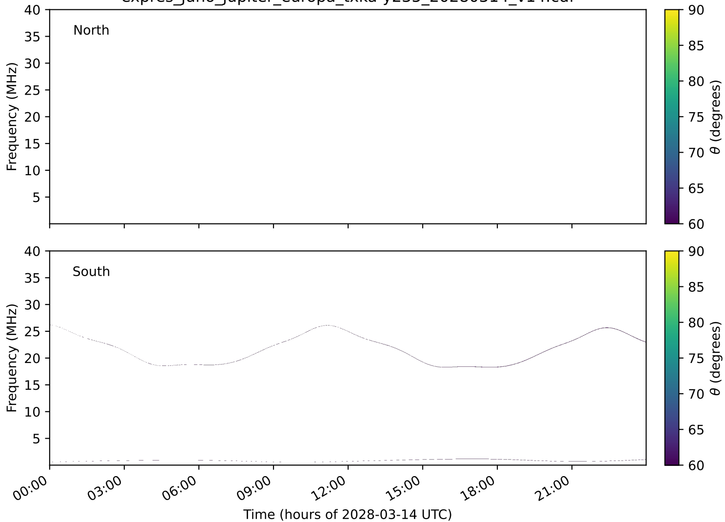
expres_juno_jupiter_europa_txka-y235_20280314_v14.cdf
