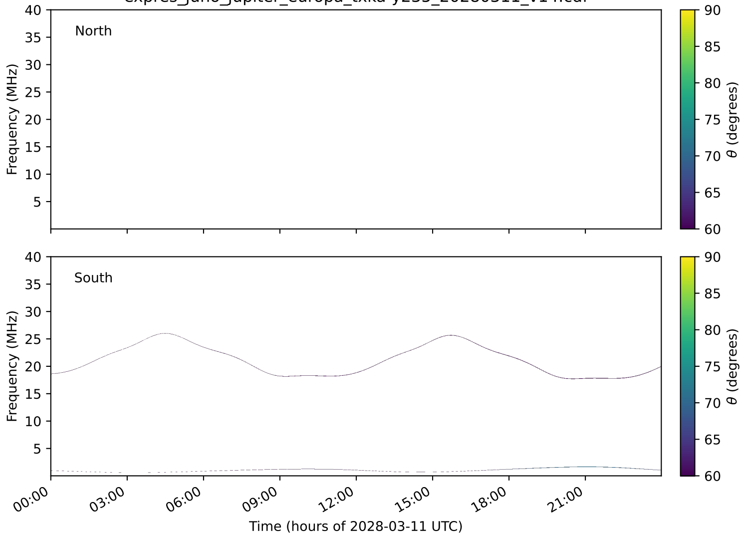
expres_juno_jupiter_europa_txka-y235_20280311_v14.cdf
