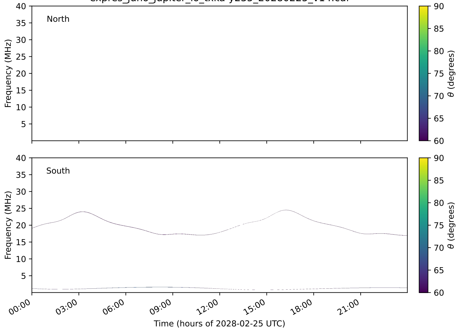
expres_juno_jupiter_io_txka-y235_20280225_v14.cdf
