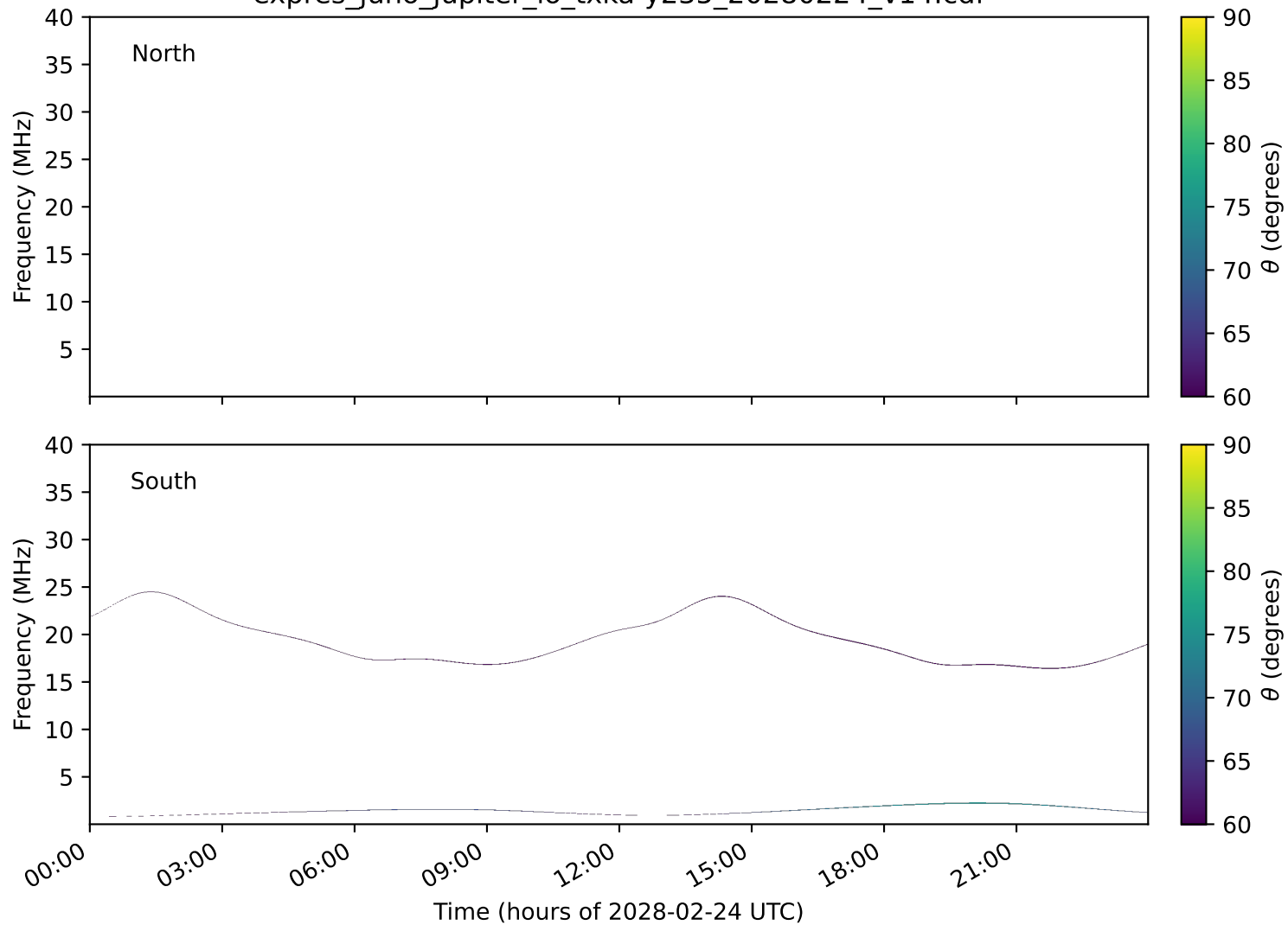
expres_juno_jupiter_io_txka-y235_20280224_v14.cdf
