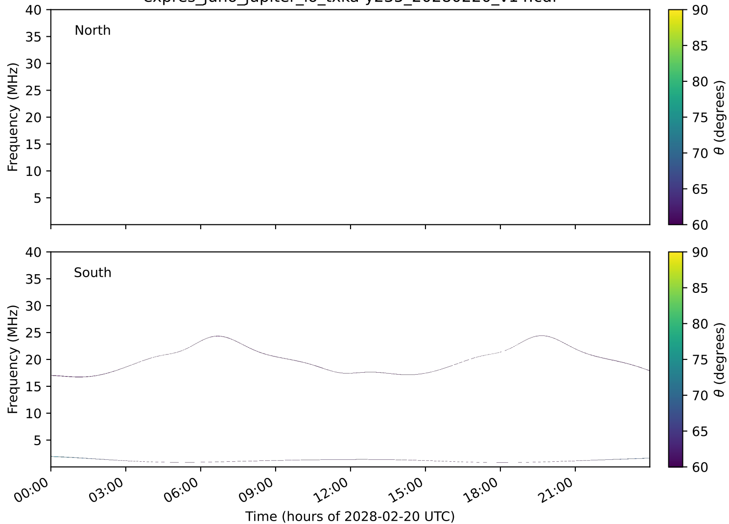
expres_juno_jupiter_io_txka-y235_20280220_v14.cdf
