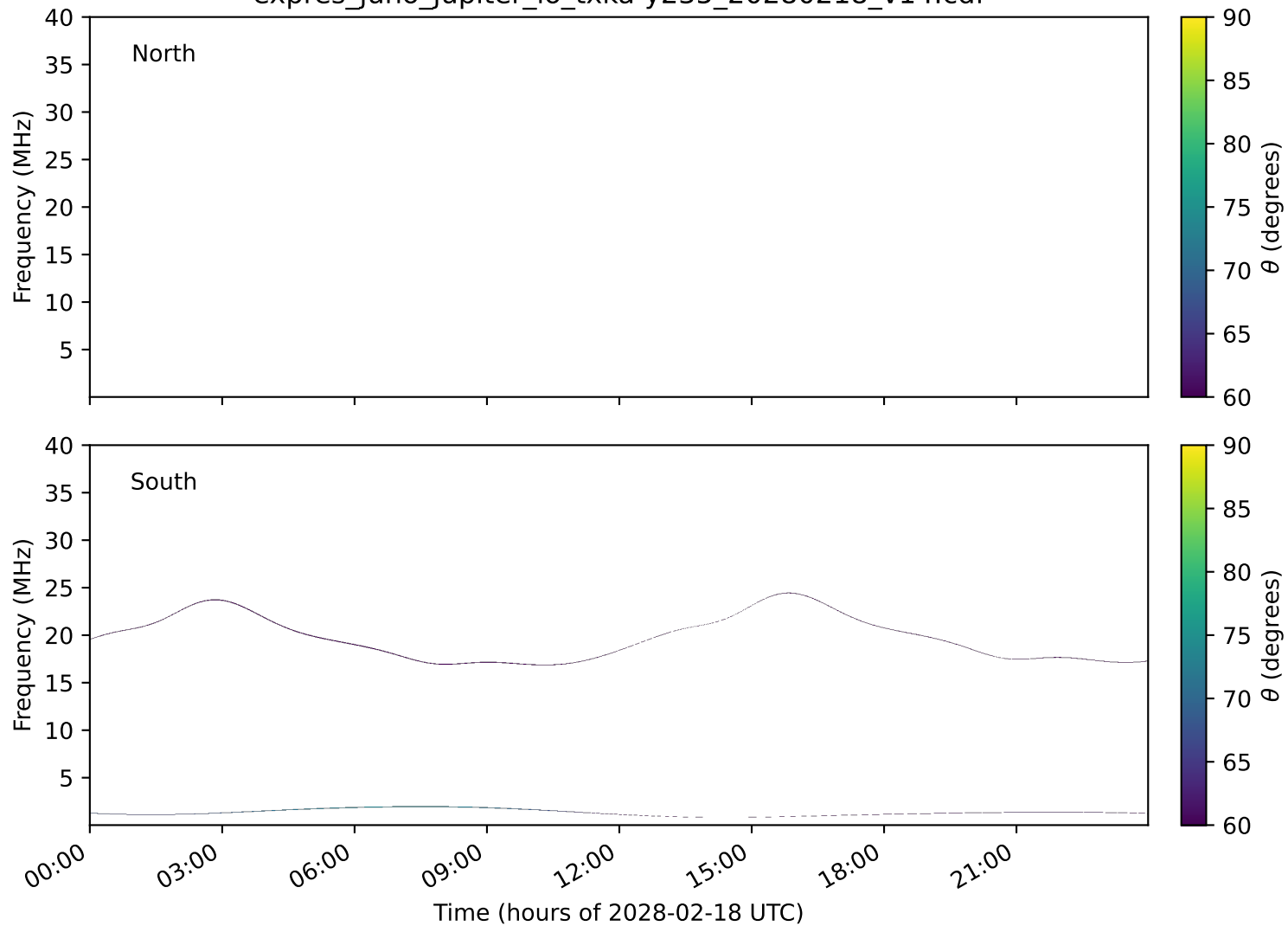
expres_juno_jupiter_io_txka-y235_20280218_v14.cdf
