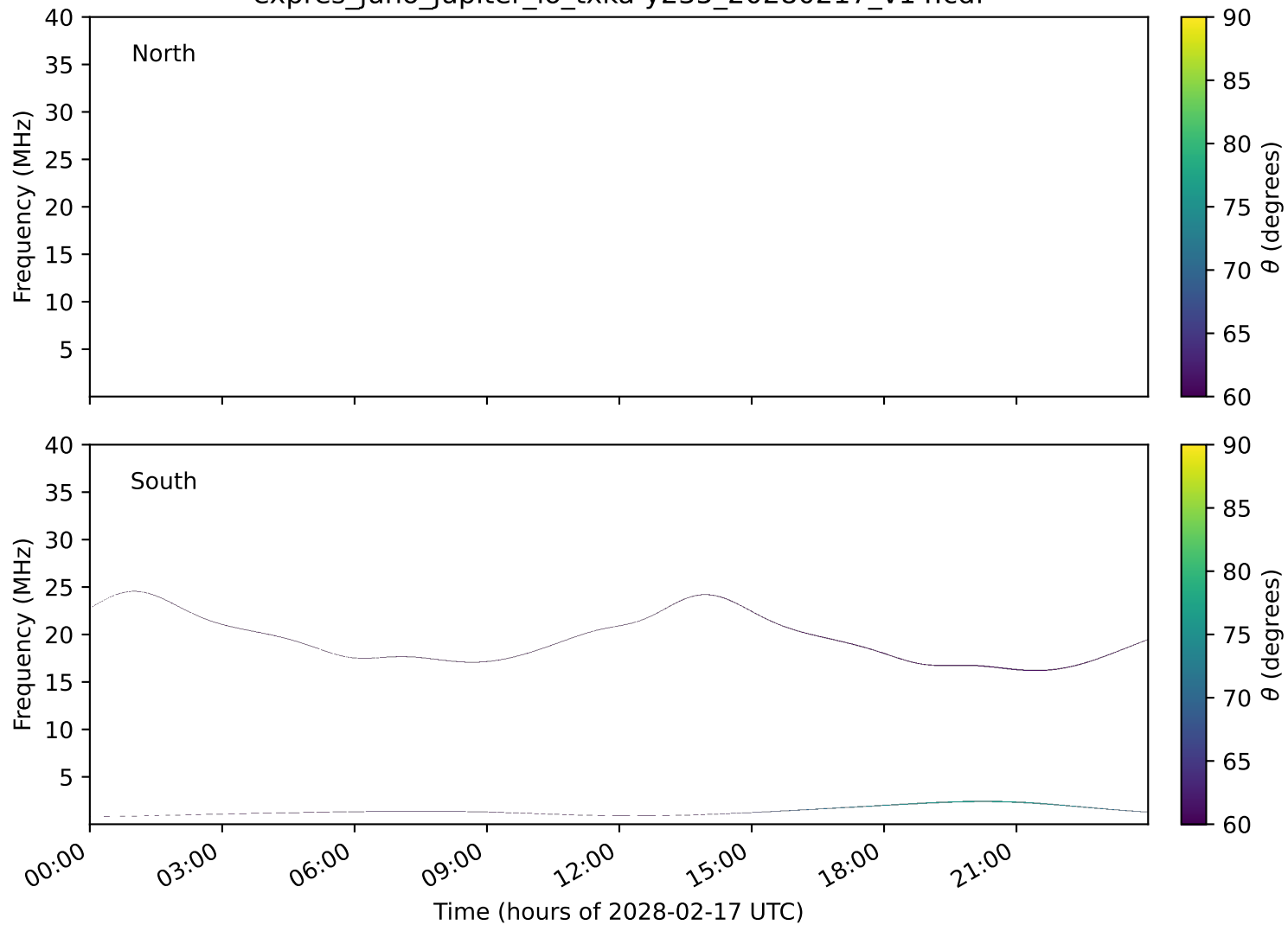
expres_juno_jupiter_io_txka-y235_20280217_v14.cdf
