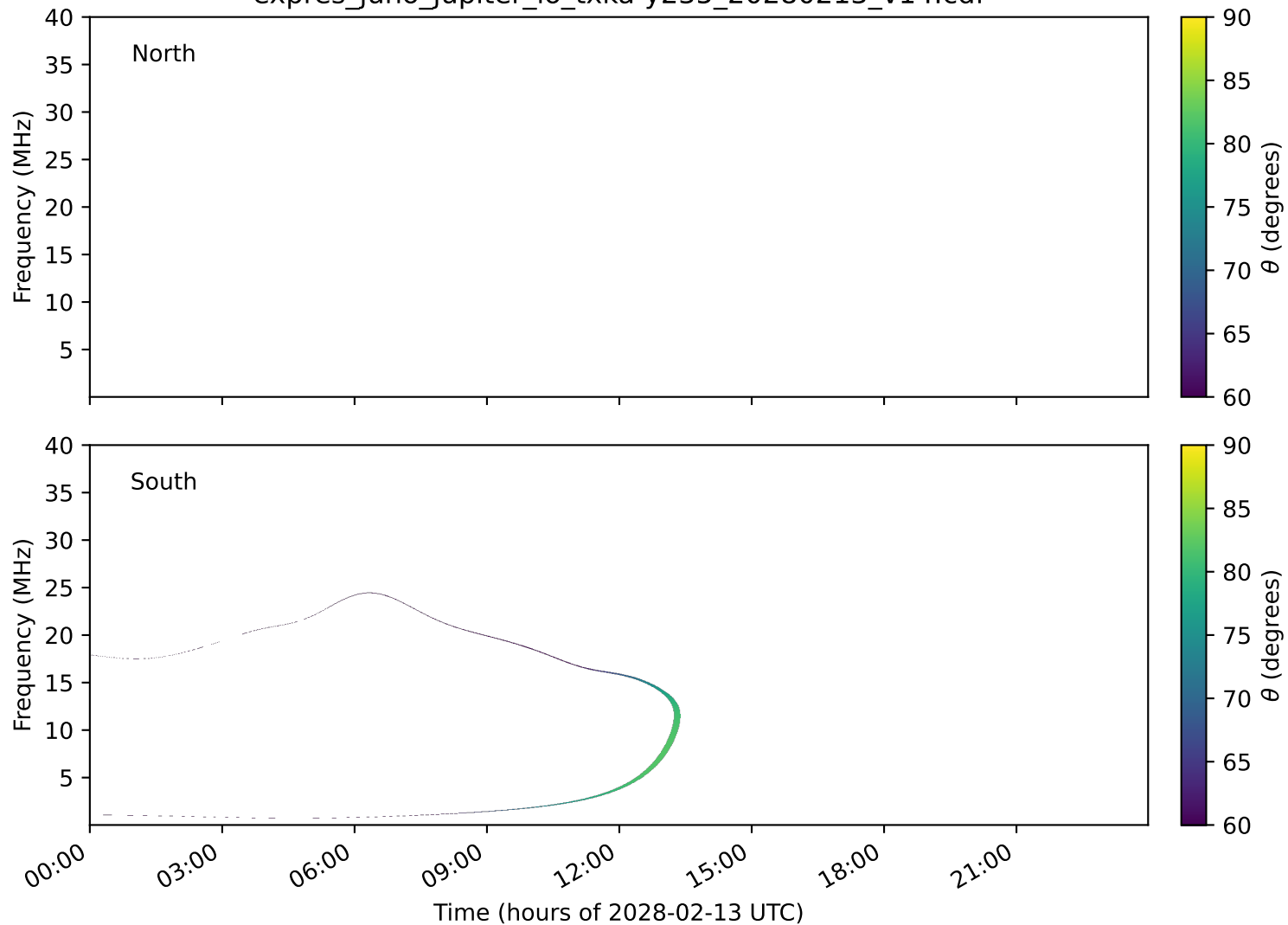
expres_juno_jupiter_io_txka-y235_20280213_v14.cdf
