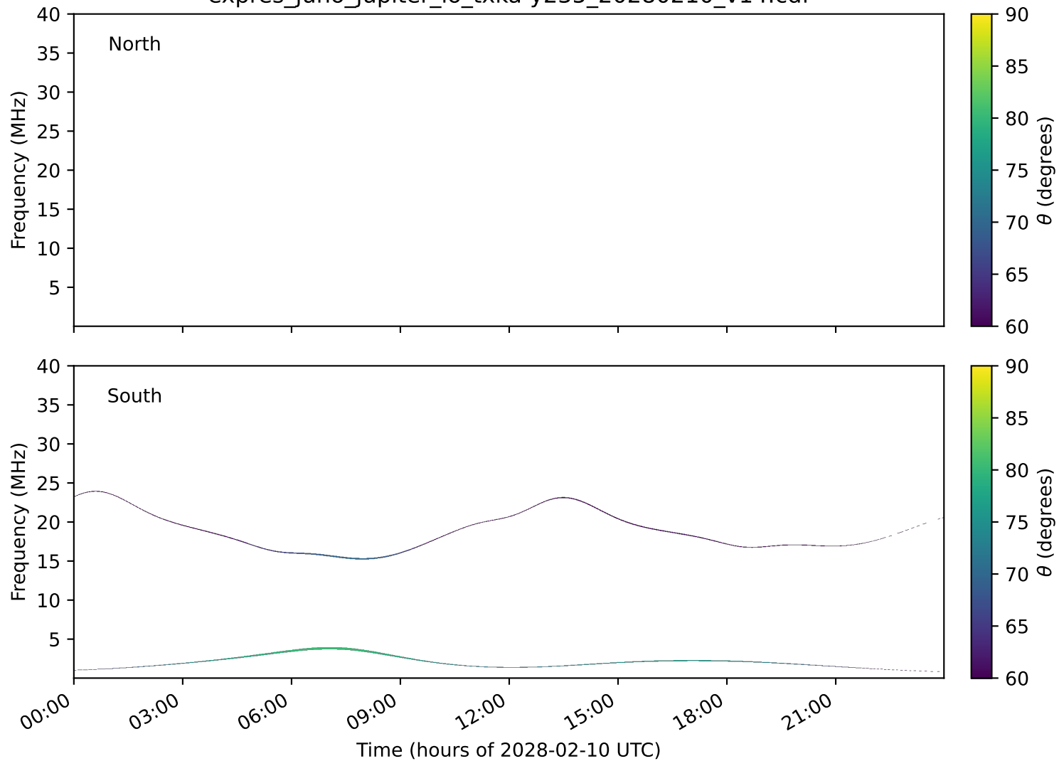
expres_juno_jupiter_io_txka-y235_20280210_v14.cdf
