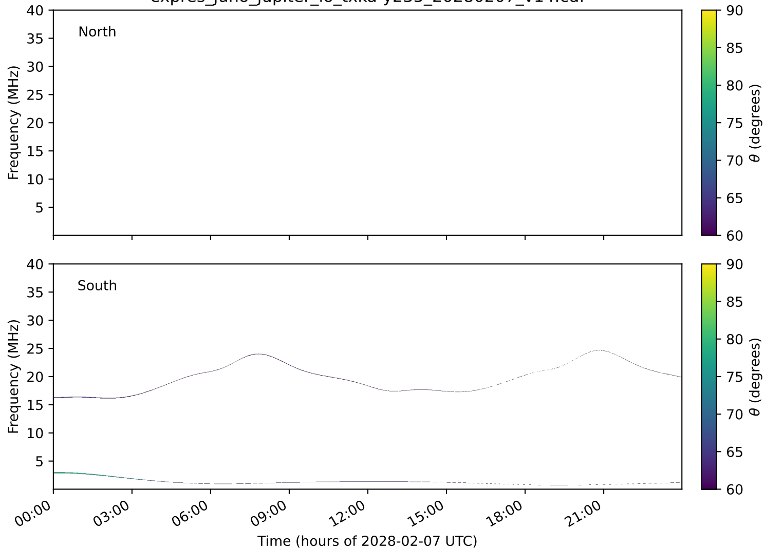
expres_juno_jupiter_io_txka-y235_20280207_v14.cdf
