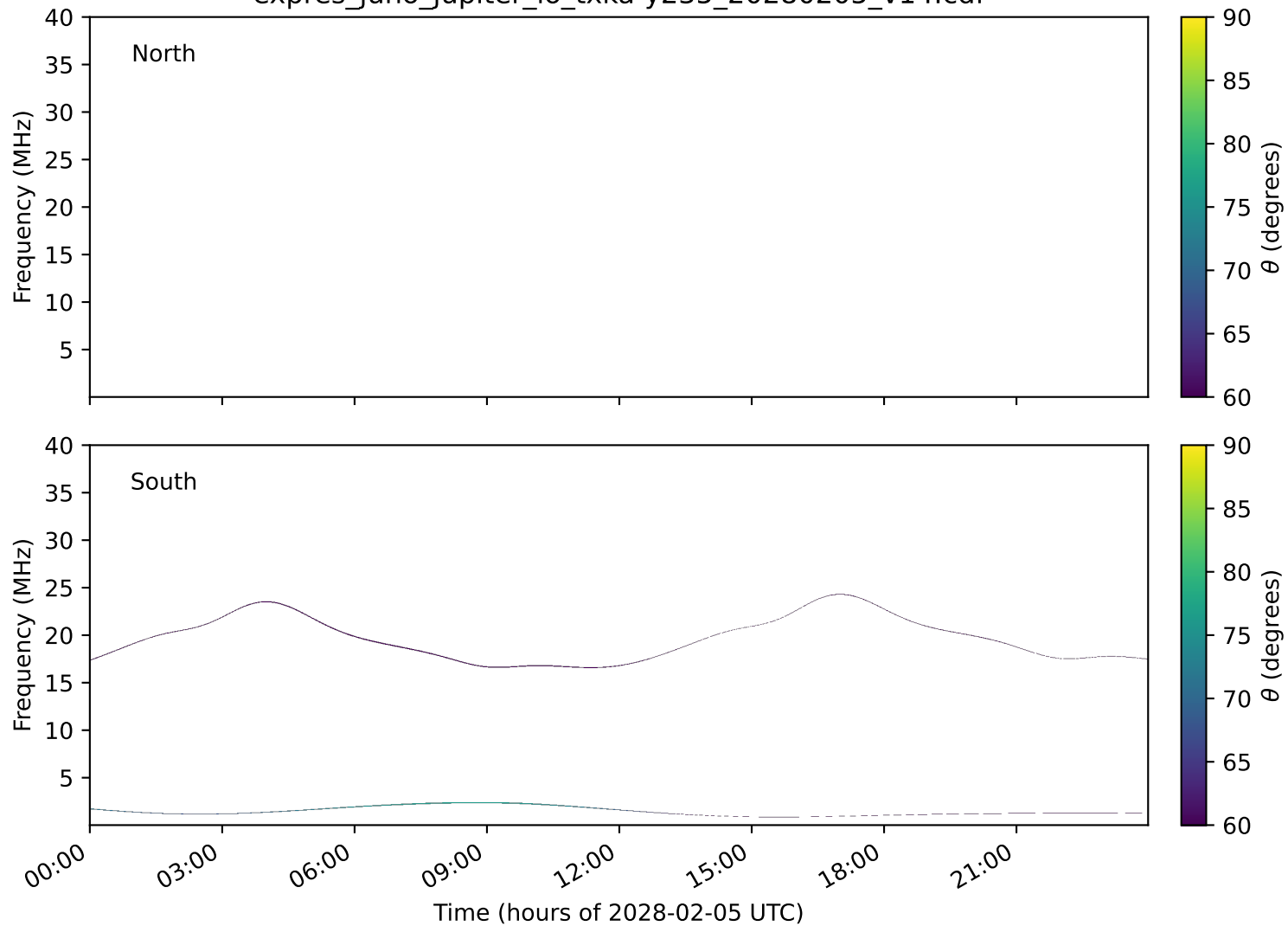
expres_juno_jupiter_io_txka-y235_20280205_v14.cdf
